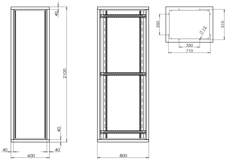
Product dimension in mm. VRF-42
